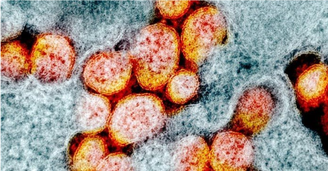
SARS-CoV-2 virus particles, isolated from a patient and imaged using a transmission electron micrograph.
